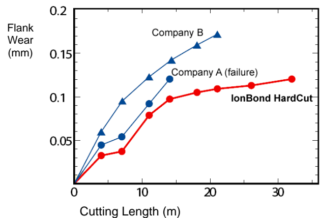
Flank Wear (mm) and cutting Length (m)
